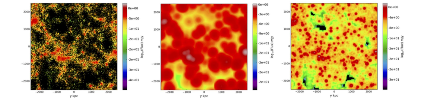
Fig 2: the left panel shows an n -body simulation of a 64 Mpc 3 volume at z=1, the middle panel shows how the volume would look to Herschel, while the right panel shows how the volume would look to a 15m FIRS. This demonstrates that while Herschel only picks up the densest nodes, FIRS obtains individual detections along the cosmic web. A FIRS also provides the spectroscopic redshifts that allow such structures to be fully characterized in three dimensions.
