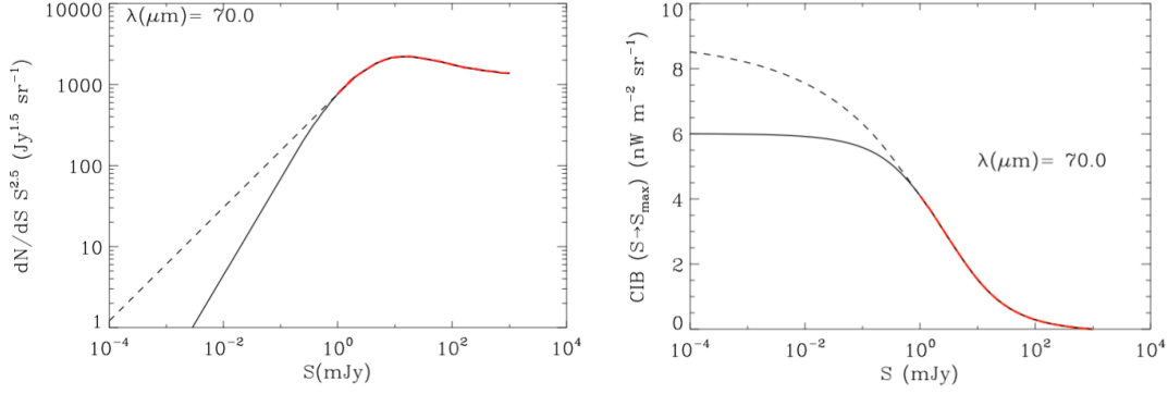
3. Figure 1: Left panel: Two different extrapolation of the Euclidean-normalized differential number counts given by Bethérmin et al. (2011). The red portion of the curve represents the contribution of resolved sources. The solid line is an extrapolation of the source counts using, in part, stacking analysis. It predicts few faint sources, and suggest that the CIB (right panel) has converged to a value of 6 \text{ nW m}^{-2} \text{ sr}^{-1} . The dashed line gives an alternative extrapolation of the number counts, producing more faint sources. In this scenario, the CIB is still increasing. Both extrapolations are within the errors of the number counts and stacking analysis. Observations at the confusion limit of a \geq 10\text{m} telescope will be able to distinguish between the two scenarios.
